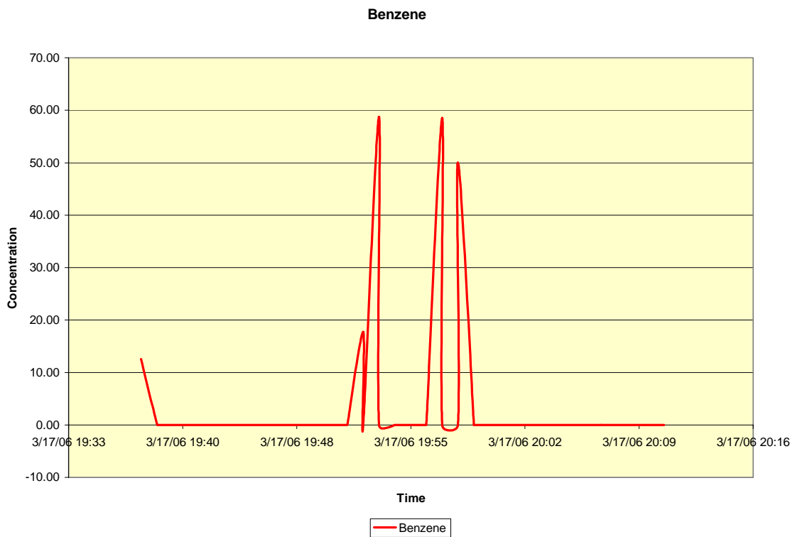
Figure 1 Benzene
