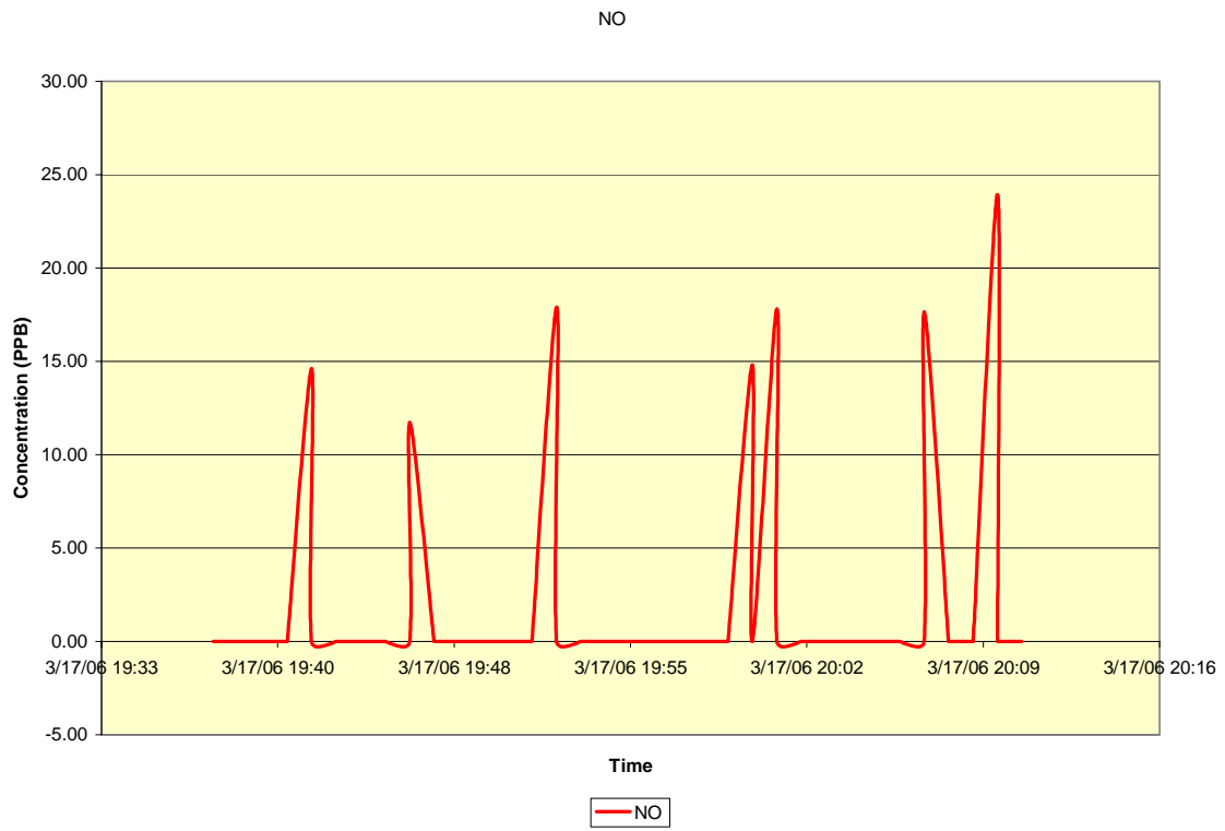
Figure 3 NO
