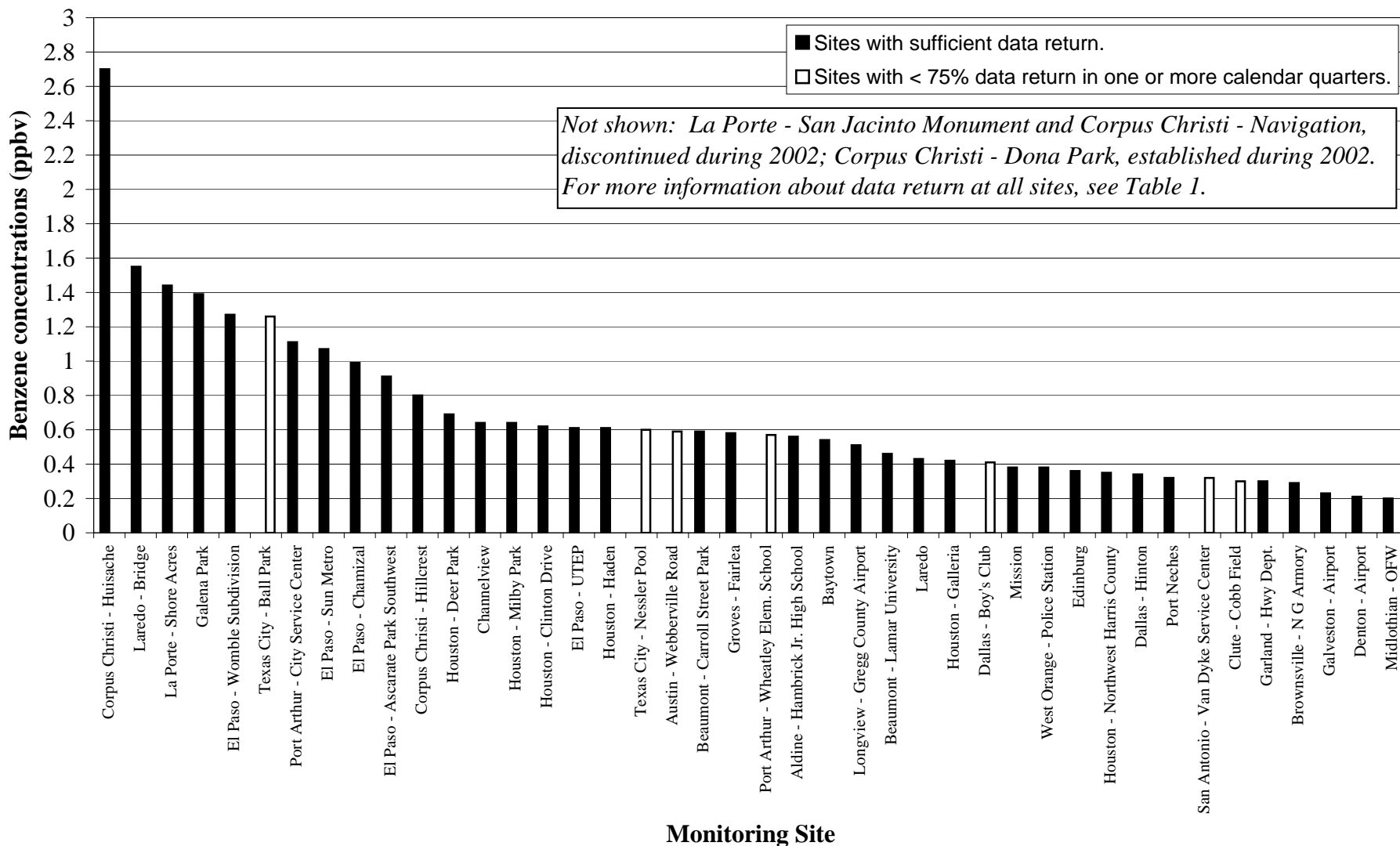
Figure 1. 2002 Annual Average Benzene Levels in Texas TCEQ Community Air Toxics Monitoring Network
